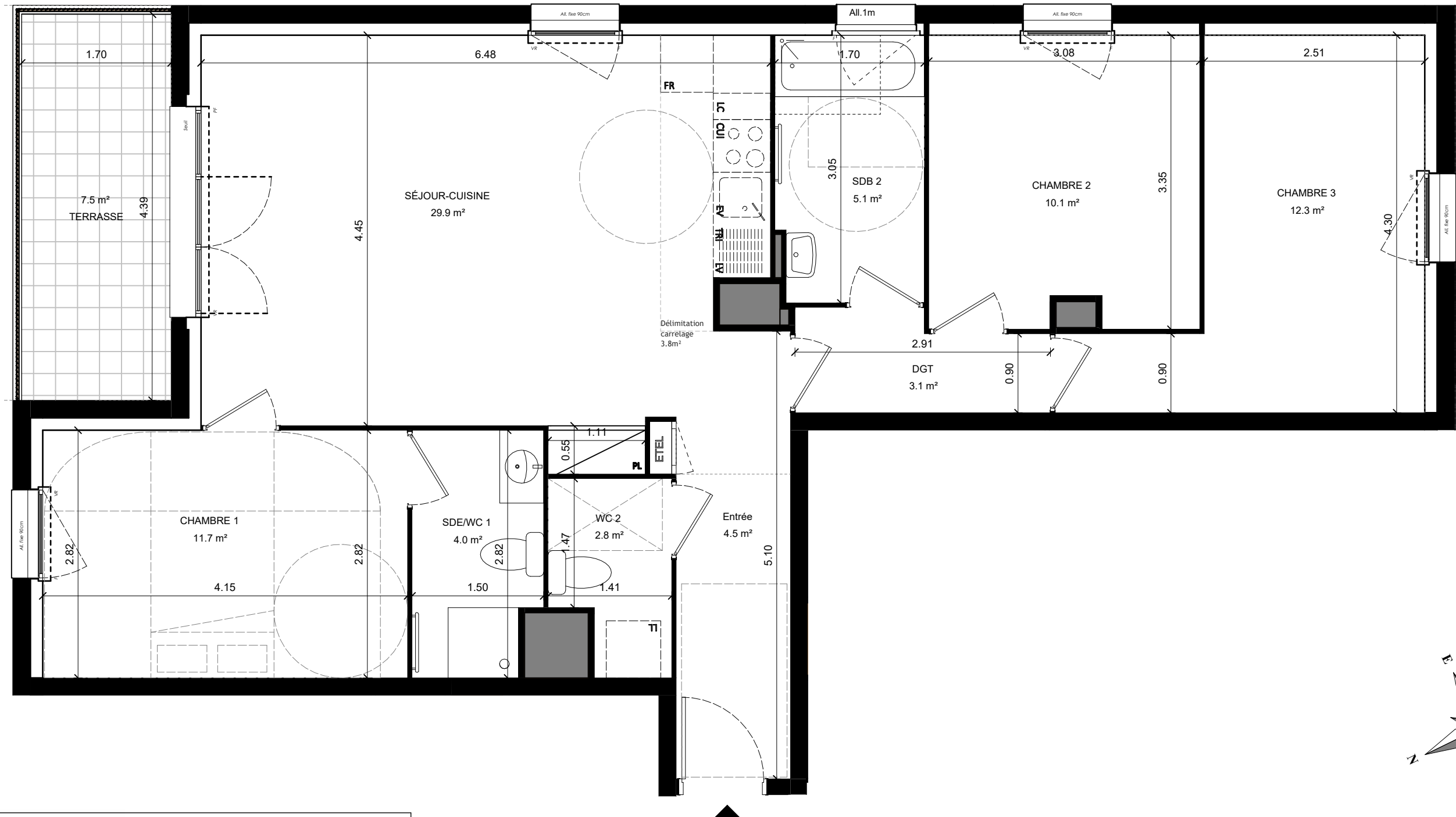
BATIMENT A
